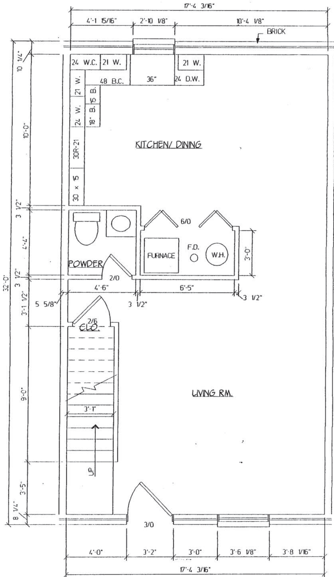
APARTMENT 'A' LOWER LEVEL FLOOR PLAN
